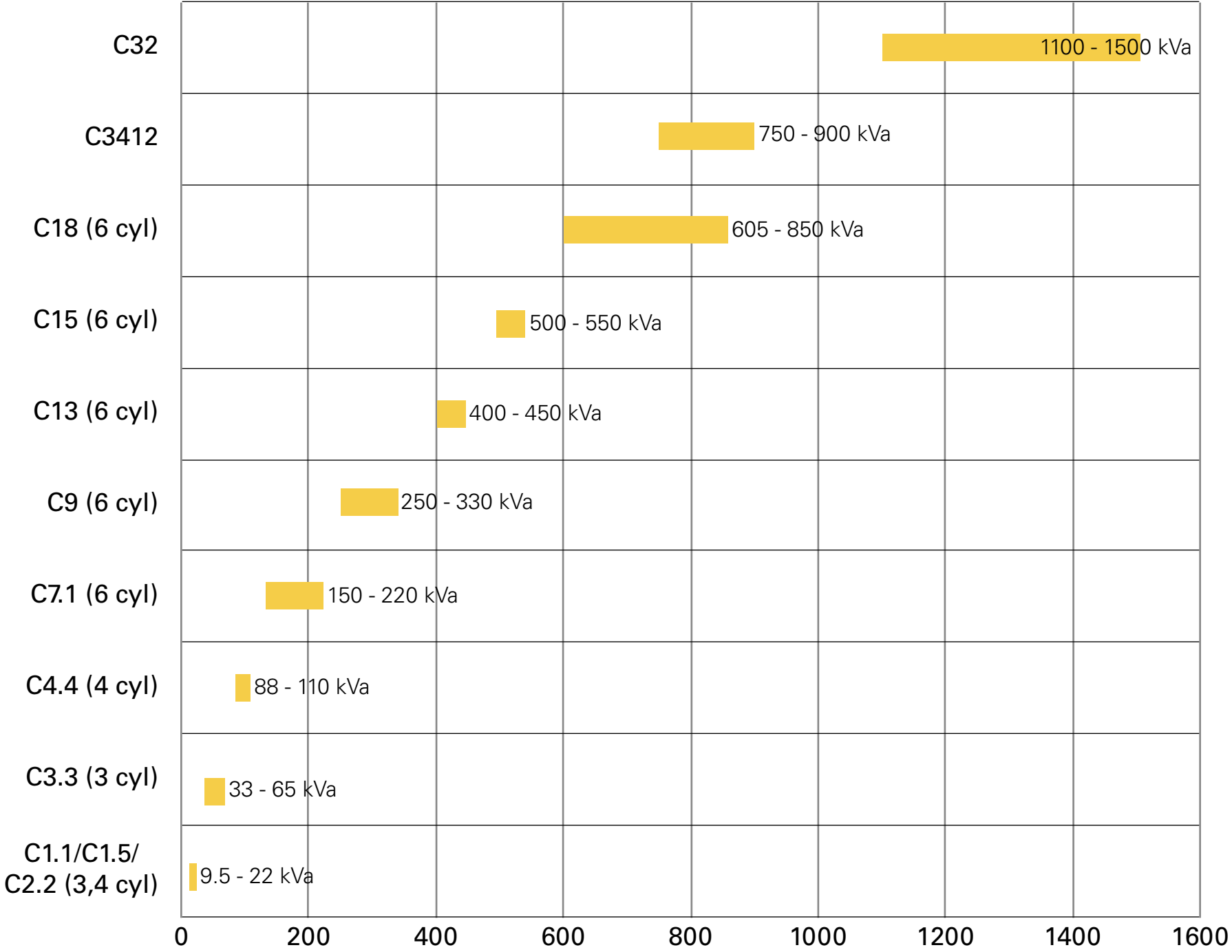
Standby power rating (50 Hz)
